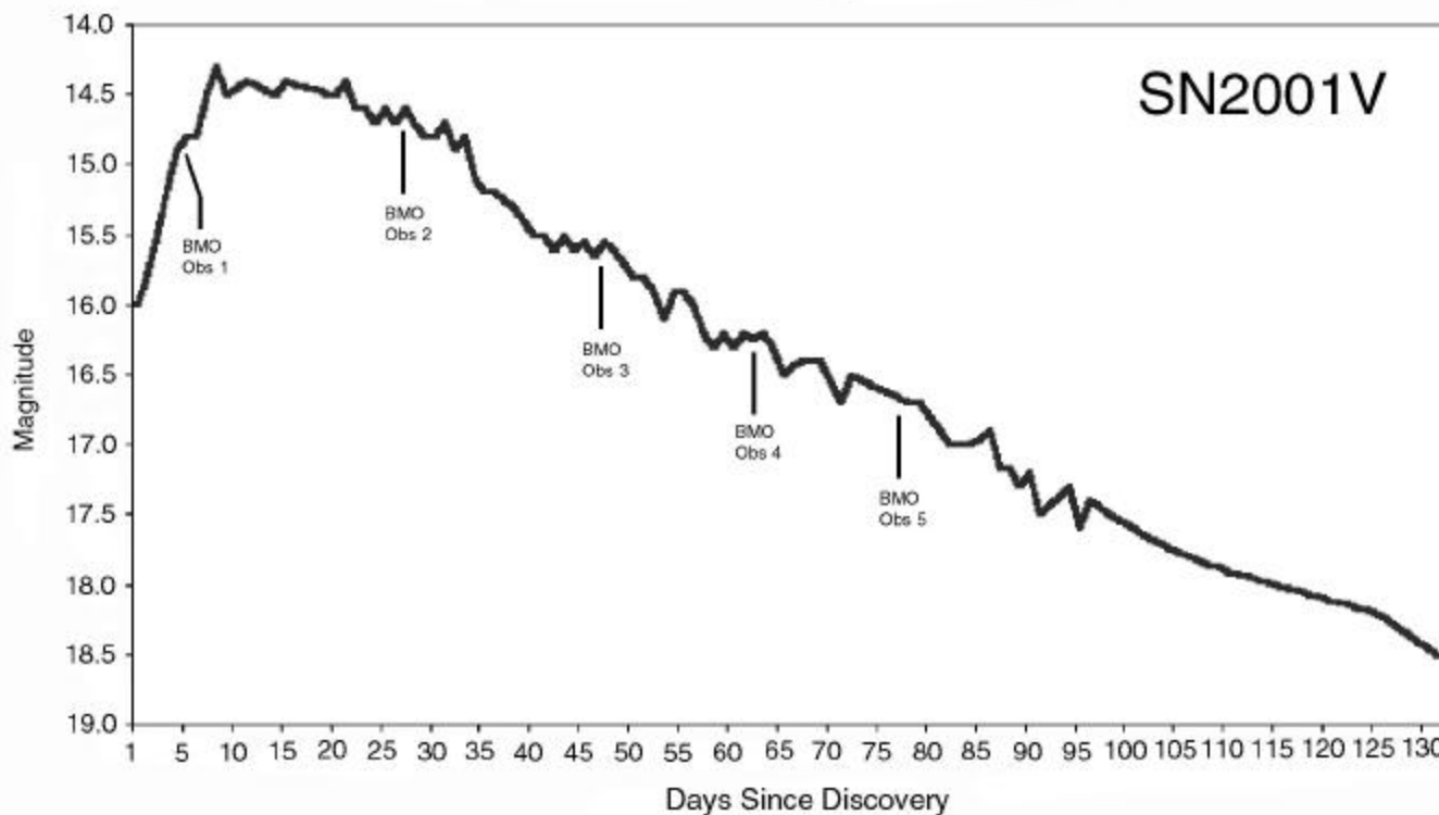
Figure 1: Typical type-Ia light curve.
