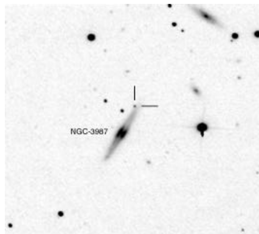
Figure 2: BMO image of SN2001V.
